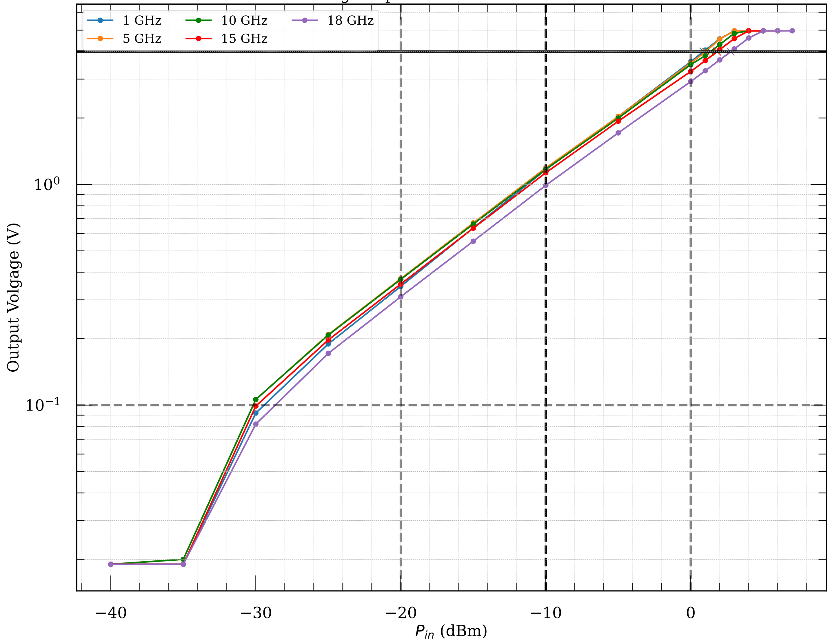
Measured voltage-to-power curve of detector module054v2
